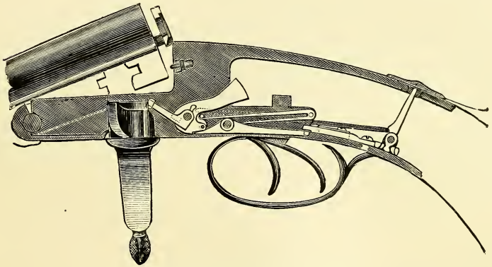
Allport's Double grip Hammerless Gun.
